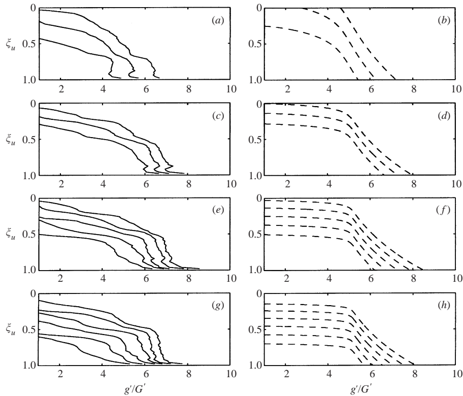
FIGURE 11. The experimental results (a, c, e, g) and numerical calculations (b, d, f, h) for the dimensionless reduced gravity in the unforced chamber. (a, b) R_A = 1 and non-dimensional time interval \Delta\tau between two adjacent lines is \Delta\tau = 3 . (c, d) R_A = 3 and \Delta\tau = 9 . (e, f) R_A = 5 and \Delta\tau = 14 . (g, h) R_A = 7 and \Delta\tau = 20 .
