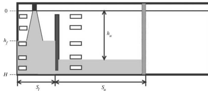
FIGURE 5. The experimental arrangement shows the forced chamber on the left and the unforced chamber on the right. A plume nozzle, located at the free surface, is placed at the centre of the left chamber. The columns of windows for measuring light intensity in both chambers are also depicted.
